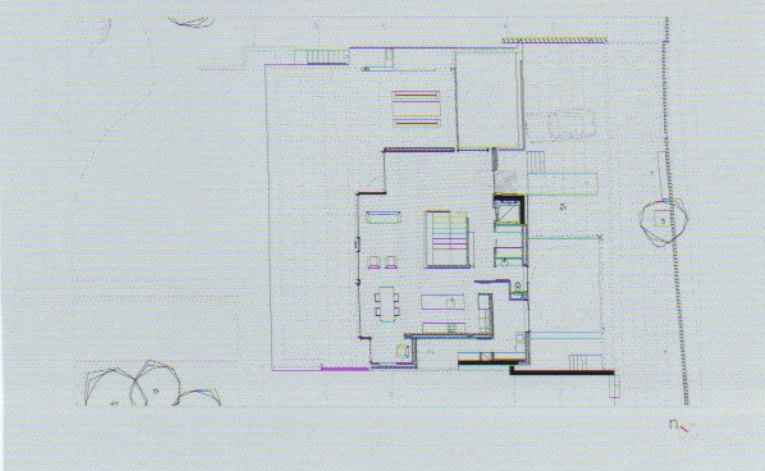
Planta baja / Ground level
